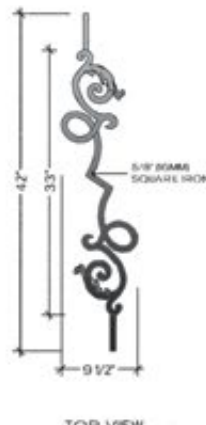
HFBX.E2
