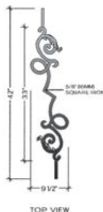
HFBX.E3
