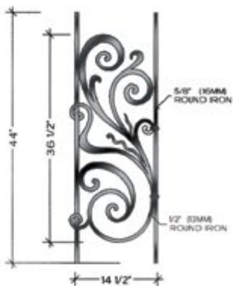
TOP VIEW A-3 ALL RADII FROM 28" TO 20'-0" HFRB.A3
