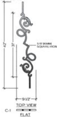
HFBX.C1
