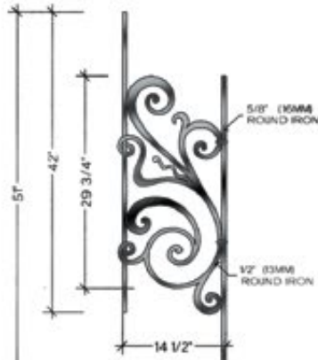
TOP VIEW B-2 ALL RADII FROM 30" TO 20'-0" HFRB.B2
