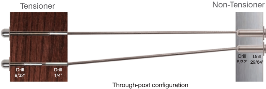
Through-post configuration
