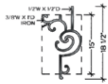
C-2 TOP VIEW ALL RADIUS FROM 30° TO 20°-0' HFRE.C2
