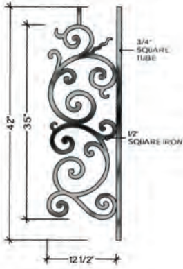
TOP VIEW FLAT A-1 HFMO.A1
