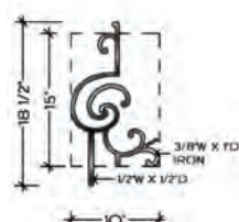
TOP VIEW C-3 ALL RADIUS FROM 30" TO 20"-0" HFRE.C3
