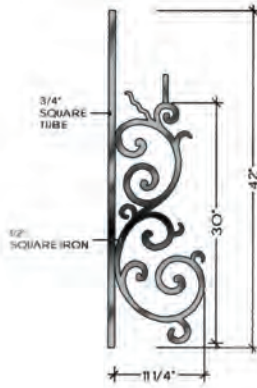
TOP VIEW FLAT B-1 HFMO.B1
