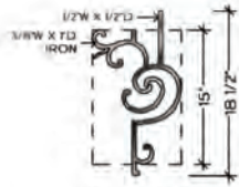
TOP VIEW C-2 ALL RADIUS FROM 30" TO 20"-0" HFRE.C2
