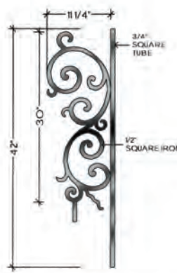
TOP VIEW B-2 ALL RADIUS FROM 30" TO 20'-0" HFMO.B2
