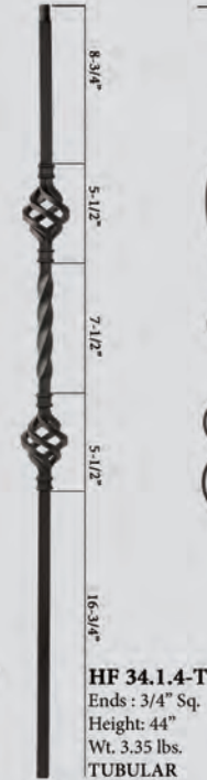
HF 34.1.3-T Ends : 3/4" Sq. Height: 44" Wt. 2.45 lbs. TUBULAR
