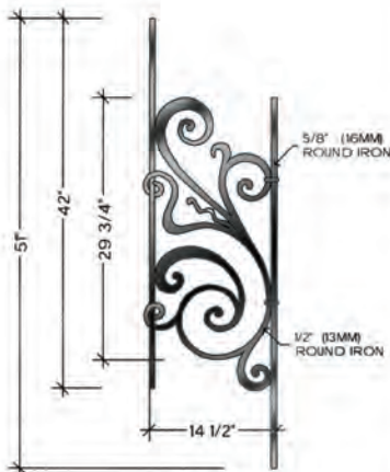
TOP VIEW B-3 ALL RADIUS FROM 30" TO 20"-O" HFRB.B3
