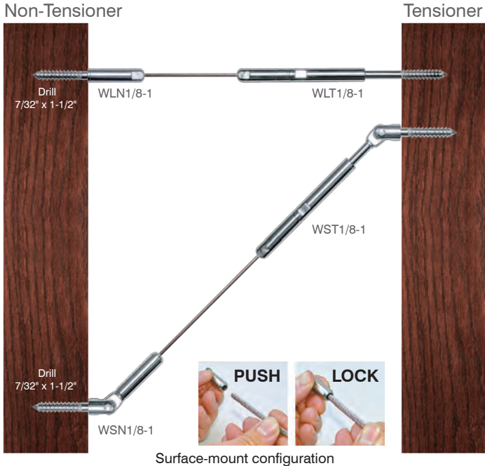
Surface-mount configuration
