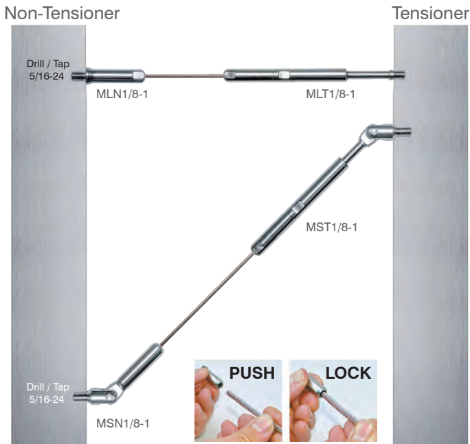
Surface-mount configuration
