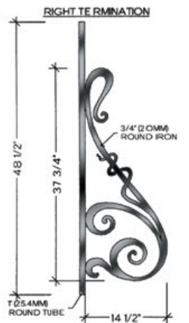
TOP VIEW 4 1/2" RADIUS HFRB.TERM RT
