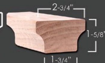
Modern Hand Rail HT. 1-3/4" W. 2-5/8"
