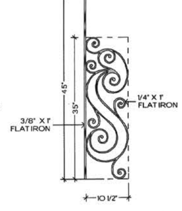
TOP VIEW D-3
