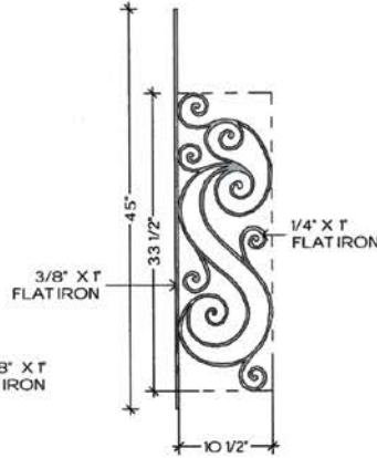
TOP VIEW C-1 FLAT
