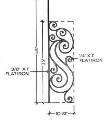
TOP VIEW D-2
