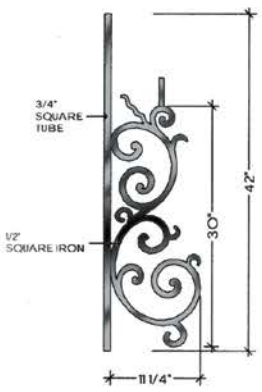
TOP VIEW B-1 FLAT HFM0.B1
