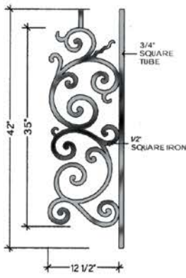
TOP VIEW A-1 FLAT HFM0.A1
