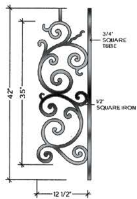
TOP VIEW A-3 ALL RADIUS FROM 28° TO 20°-0° HFM0.A3
